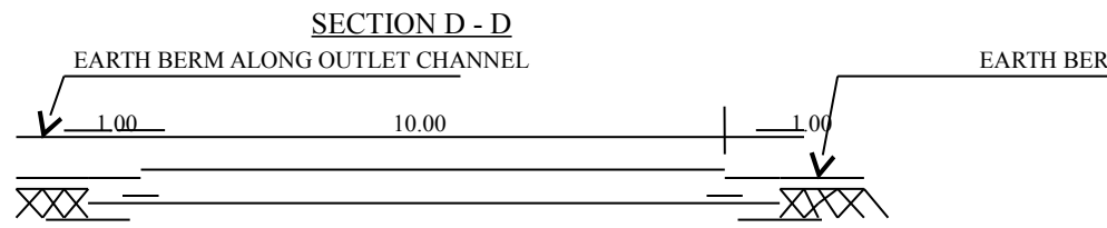
INLET TO SILT TRAP CROSS SECTION E - E
