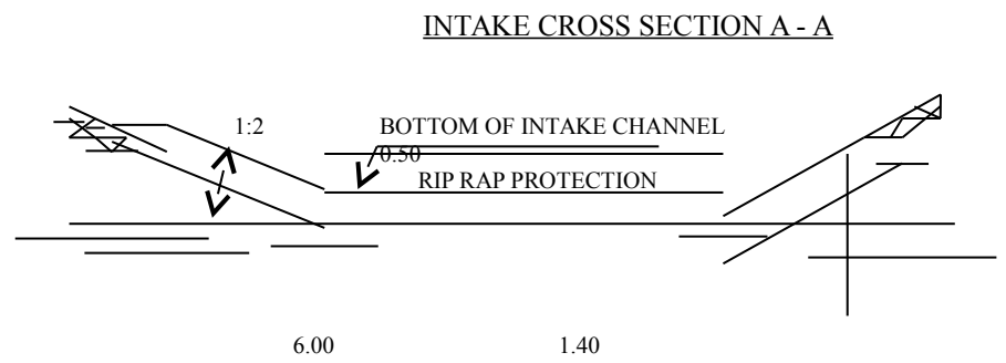
INTAKE CHANNEL SILL CROSS
